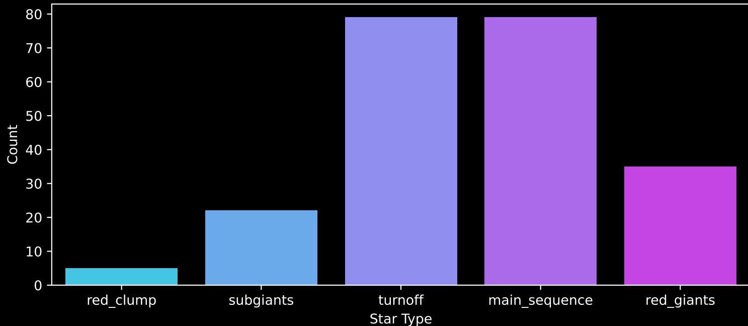
GALAH DR4 Field: [7173] Count plot of Star Type
