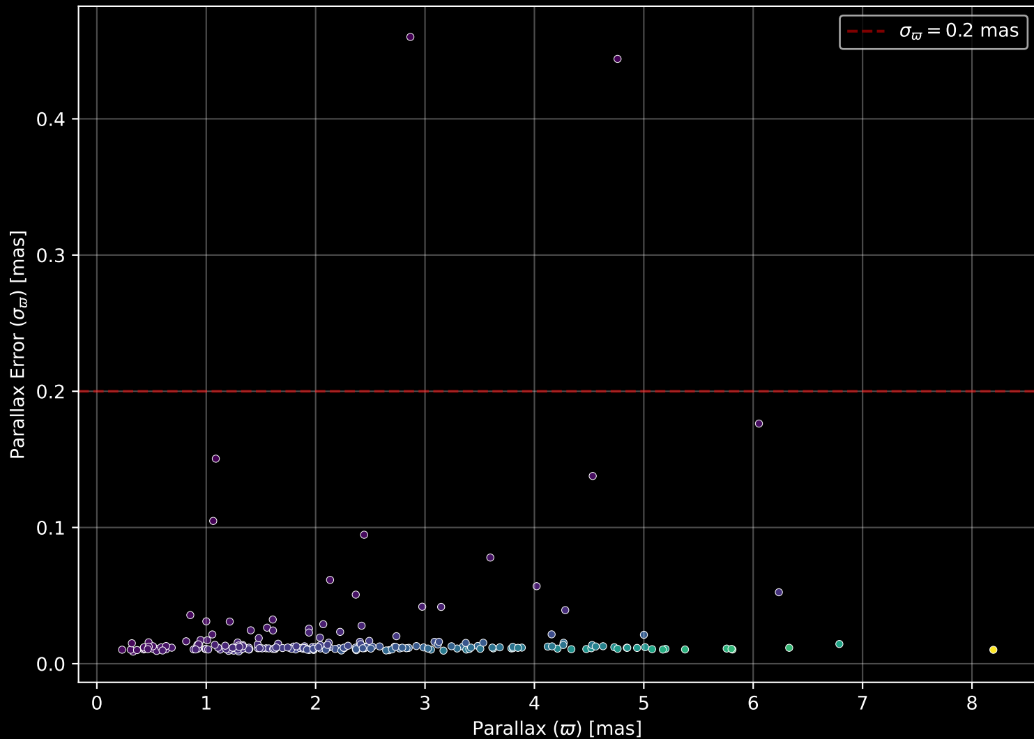
GALAH DR4 Field: [7173] Parallax Quality (n= 220)
