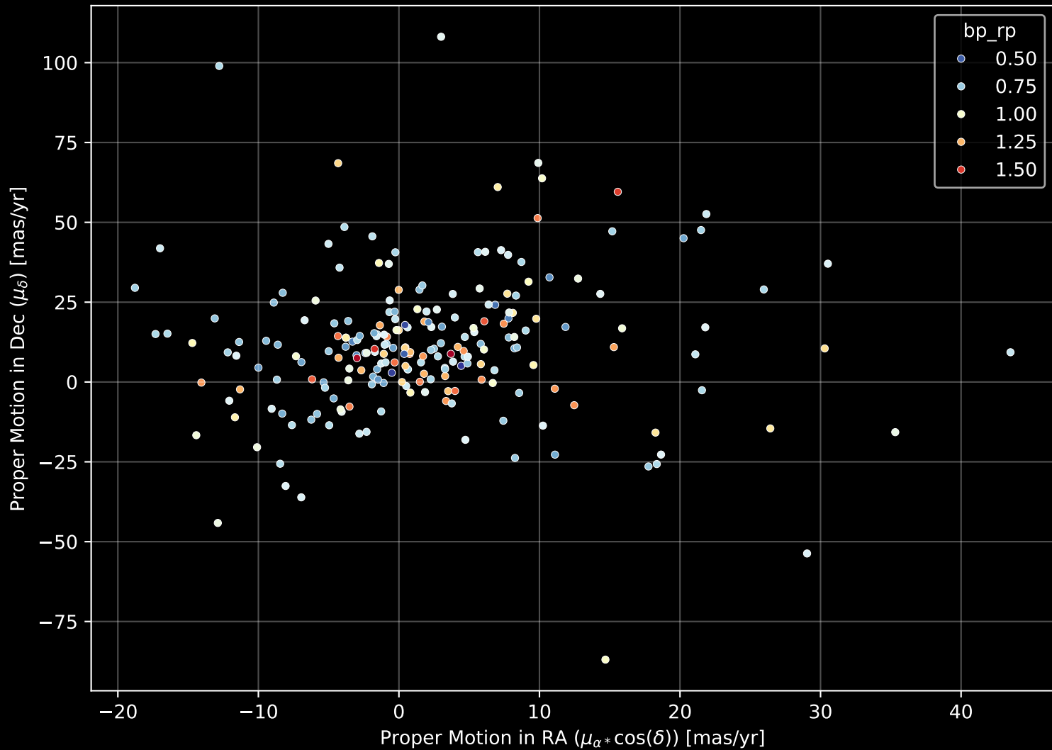
GALAH DR4 Field: [7173] Proper Motion Diagram (n= 220)
