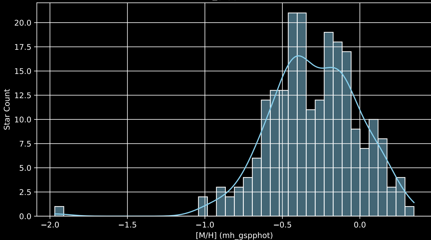
GALAH DR4 Field: [7173] [M/H] (mh_gspphot) (n= 220)
