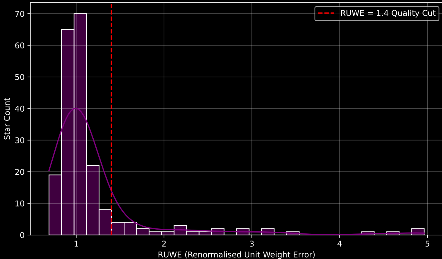
GALAH DR4 Field [7173] RUWE Distribution (n= 212)
